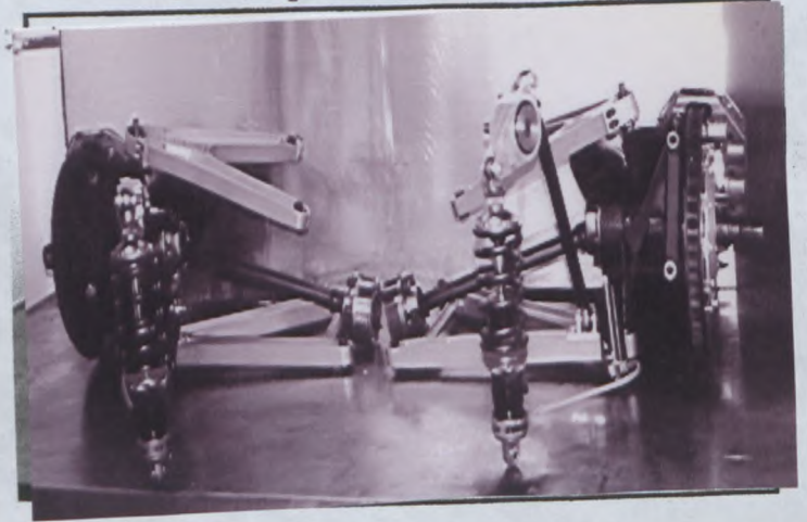
PHOTO N° U - complete rear axle
