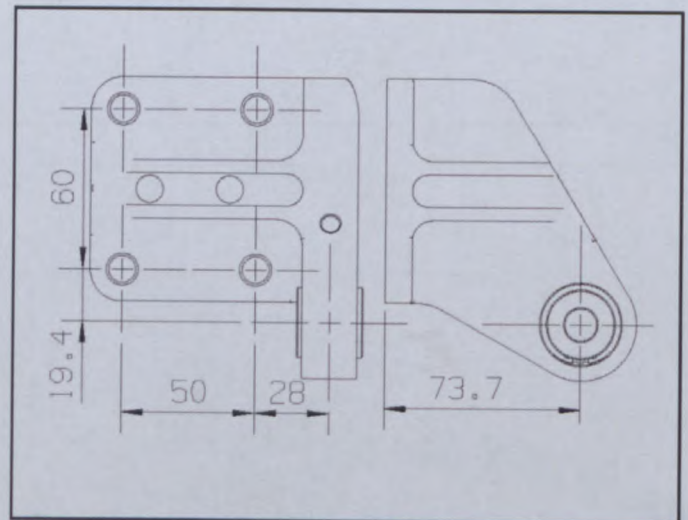
DRAWING SM3
