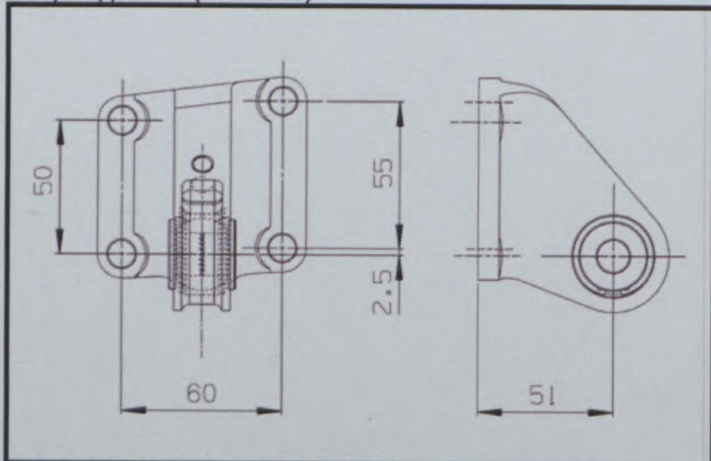
SM3) Support n°3 (DRAWING)
