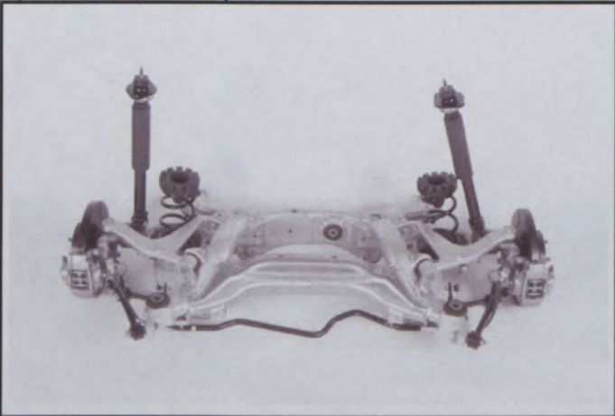
U) Rear axle assembly
