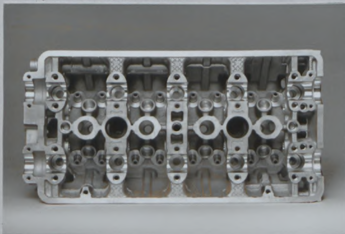
Culasse nue vue de dessous Bare cylinder head seen from above
