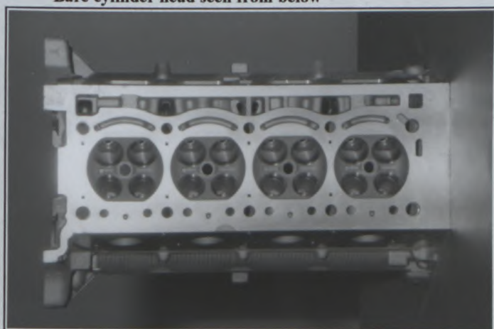
Bare cylinder head seen from below
